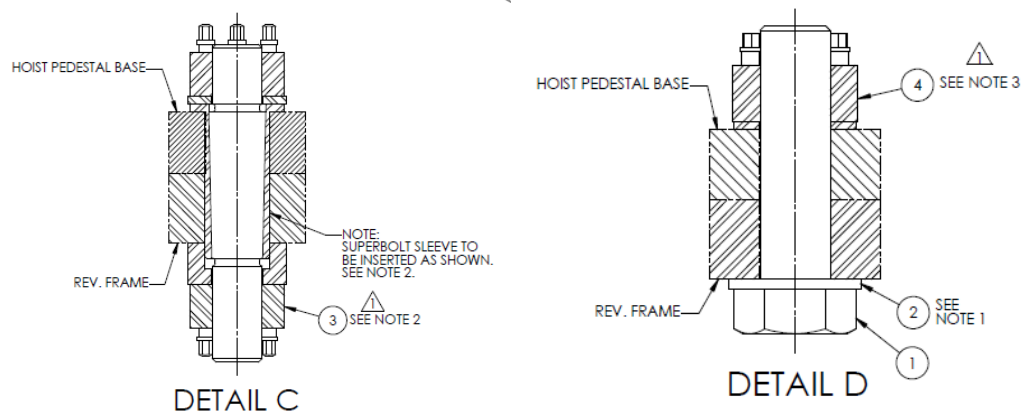
Figure 7: Super bolts detail
