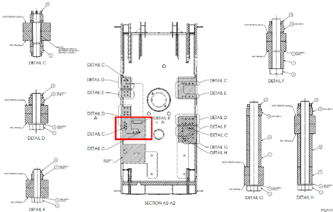
Figure 2: Location of super bolts of hoist pedestal
